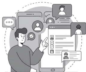
SEBI Scores
